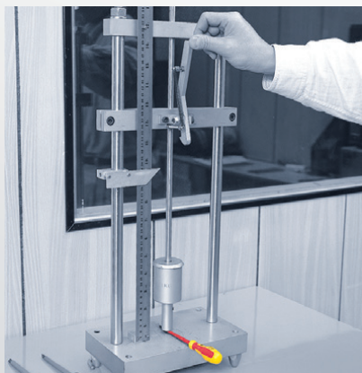
Impact Testing
